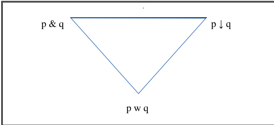
2. The logical triangle of contrariety 1 , with compound sentences
