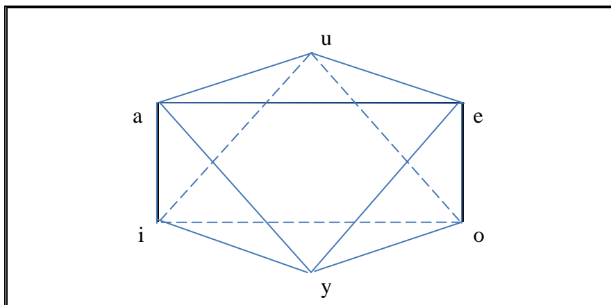
1. The oppositional hexagon of Robert Blanché
