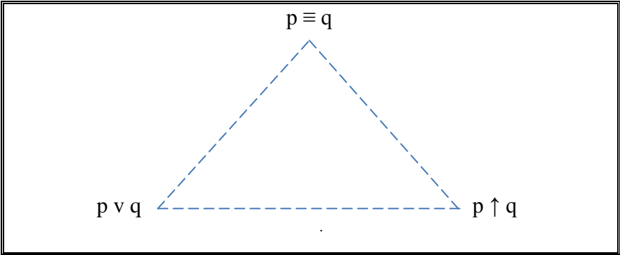
3. The logical triangle of subcontrariety 2 , with compound sentences
